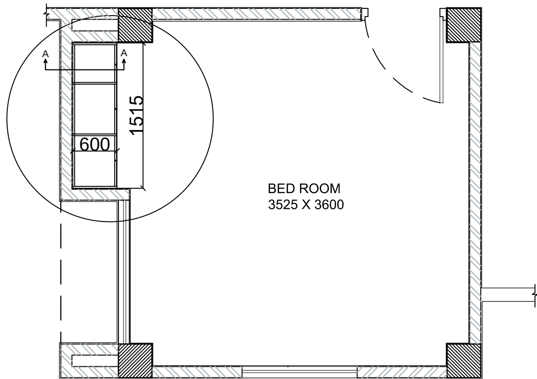
KEY PLAN (SHOWING THE CABINET)
