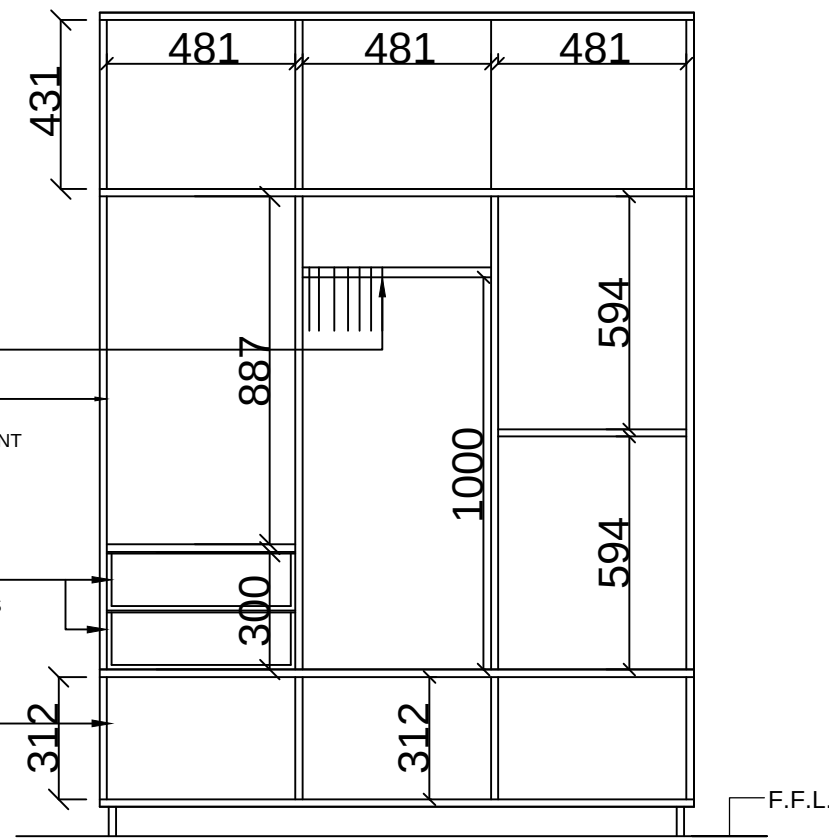
INSIDE ELEVATION
